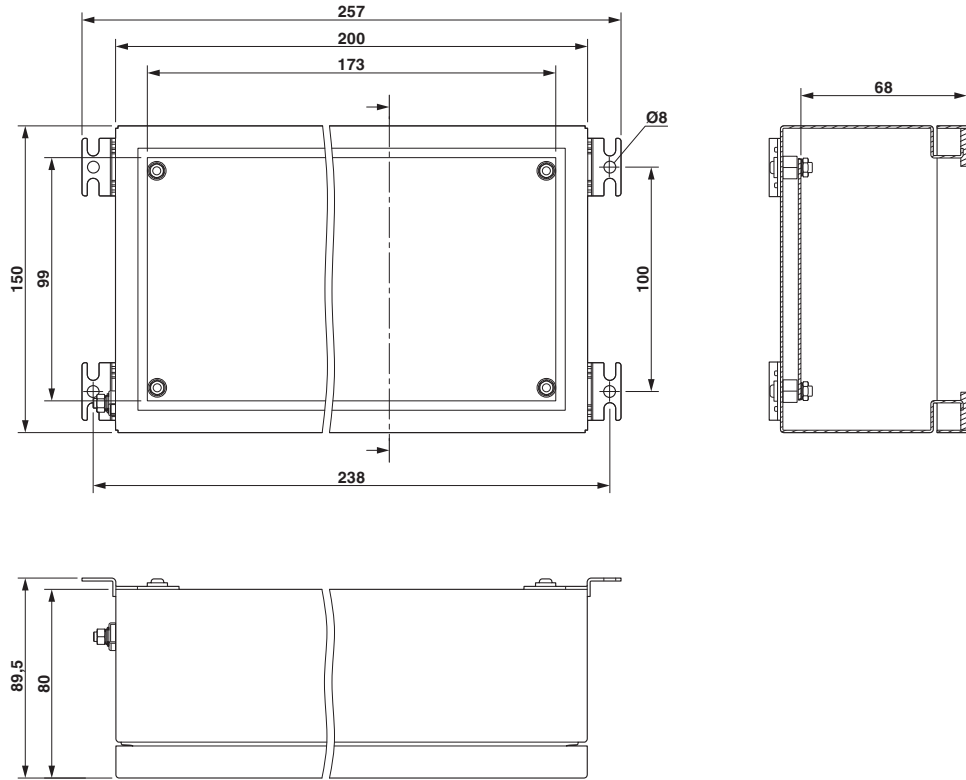
Dimensional drawing
